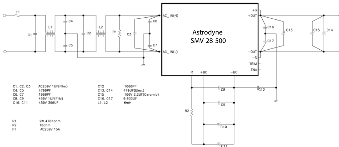
Fig. 3 Application Circuit.
