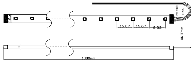
Outline Dimension
