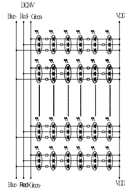
Circuit Diagram
