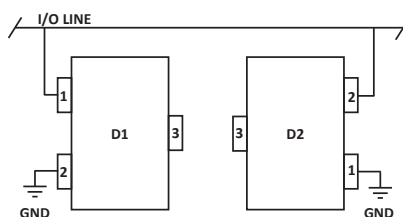
FIGURE 2 - BIDIRECTIONAL COMMON MODE PROTECTION
