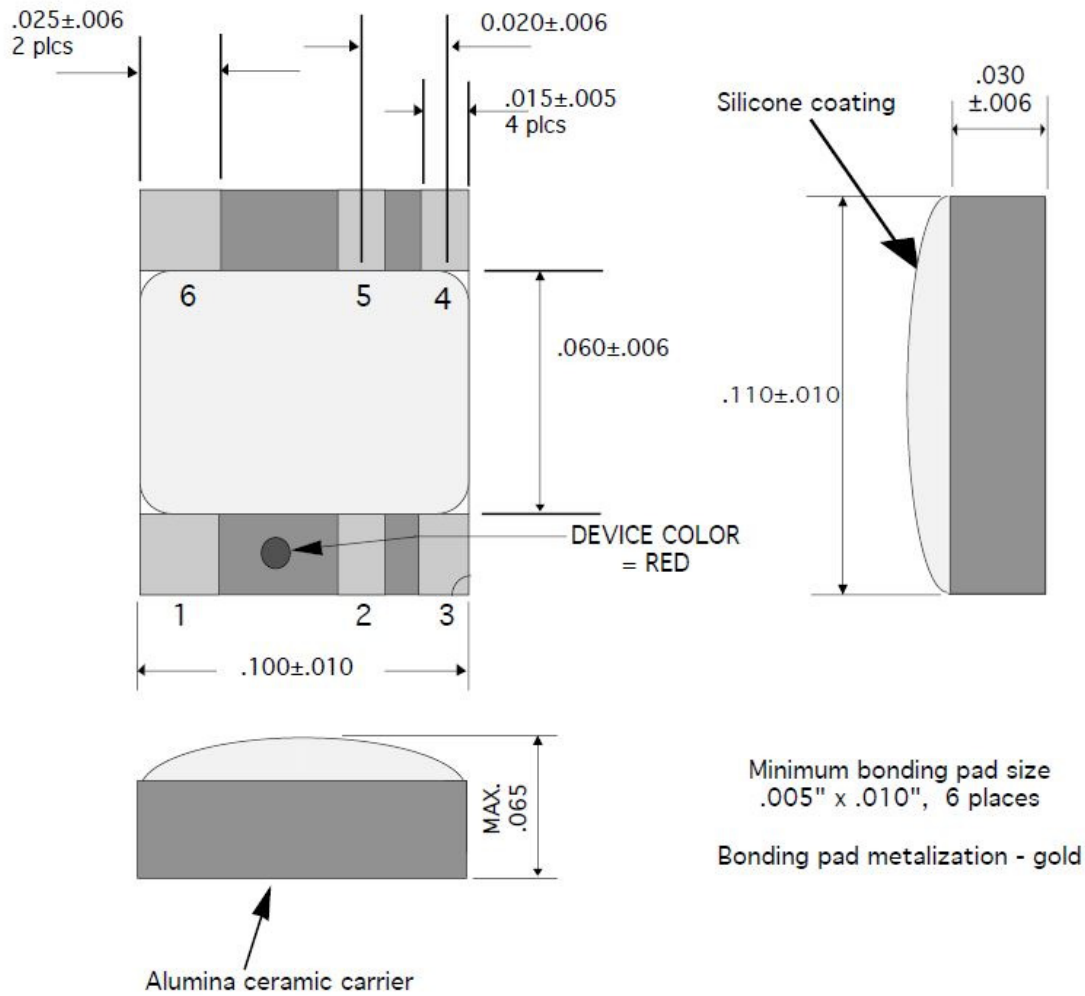
Figure 7. OLI500 Package Dimensions
