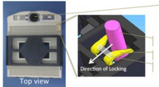
Socket for mPGA type CPU
