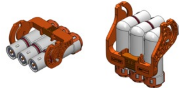
HVC 3 POLE 300A METAL HIGH VOLTAGE CONNECTOR
